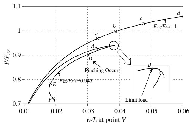
Fig. 10. Detail of two load–displacement curves of Fig. 9. Points A , B are on the loading path, C , D , E , F on the unloading one. Inset shows the peak load. Points a , b , c , d are all on the loading path.
