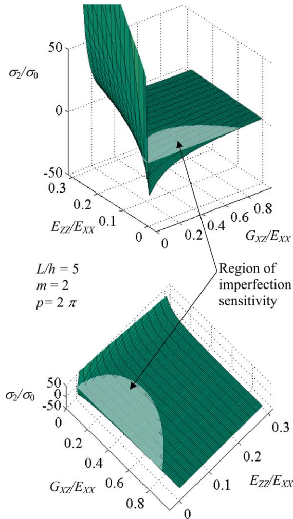
Fig. 2. Imperfection sensitivity for a short column clamped at both ends and m = 2 .
